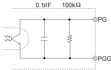
Fig.1.8 Internal circuit of PG
