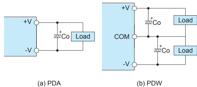
Fig.7.2 Output side external capacitor connection method
