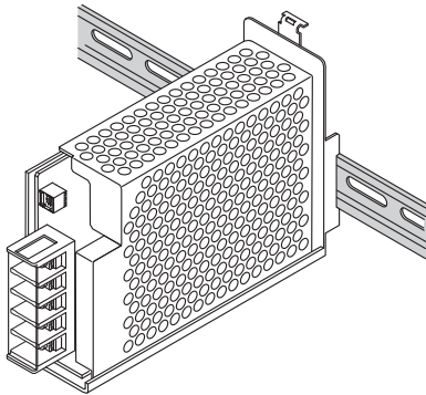
Fig.8.2 Power supply installed on a DIN rail
