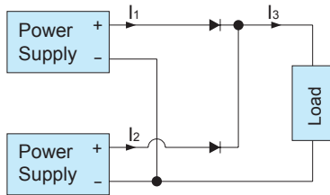
Fig.3.2 Example of redundancy operation
