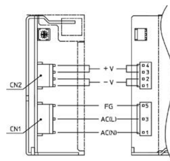
Fig.8.1 Image of option -J1 (PDA50F)
