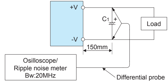
Fig.1.3 Measuring method of Ripple and Ripple Noise
