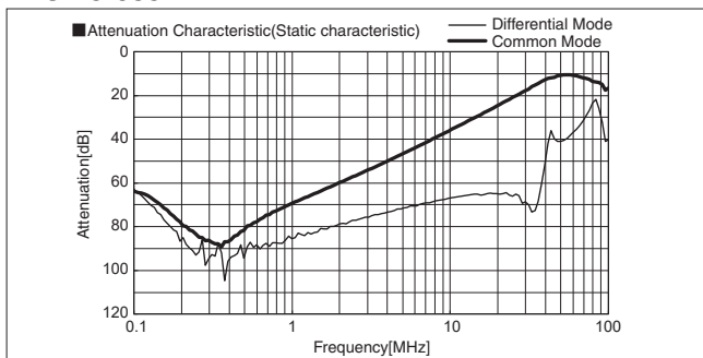
YAC-64-685
