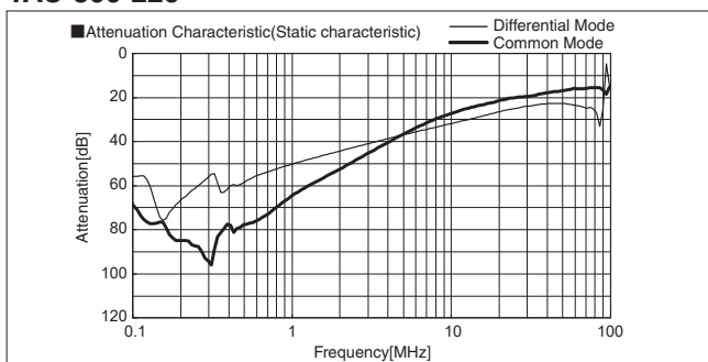
YAC-300-226
