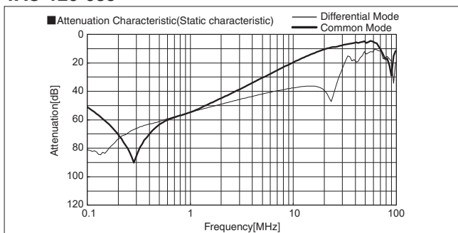
YAC-200-685
