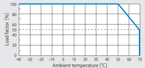
Derating curve (CXLDA480F)
